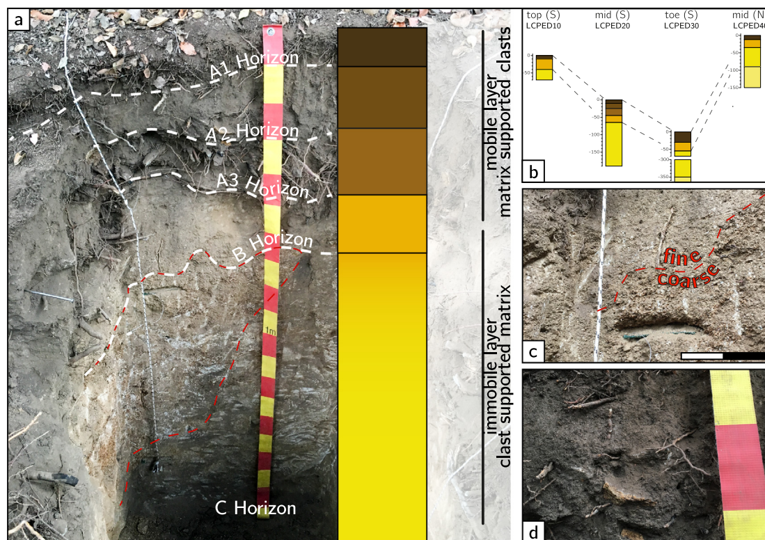
Fig. 5. Photographs of the S-facing mid slope pit (LCPED 20) in Parque Nacional La Campana (LC) including horizon boundaries (white dashed line), a profile sketch, and a cross section through the S-facing catena and adjacent N-facing pit. Both coarse- and fine-grained granodiorite comprise the substrate of the regolith (boundary shown by the red dashed line) (a); scale bar size: 10 cm. Mid slope pits (S- and N-facing) are affected by mass movement downslope, leading to an accumulation of angular fragments in the soil columns (b). (For interpretation of the references to color in this figure legend, the reader is referred to the web version of this article.)
