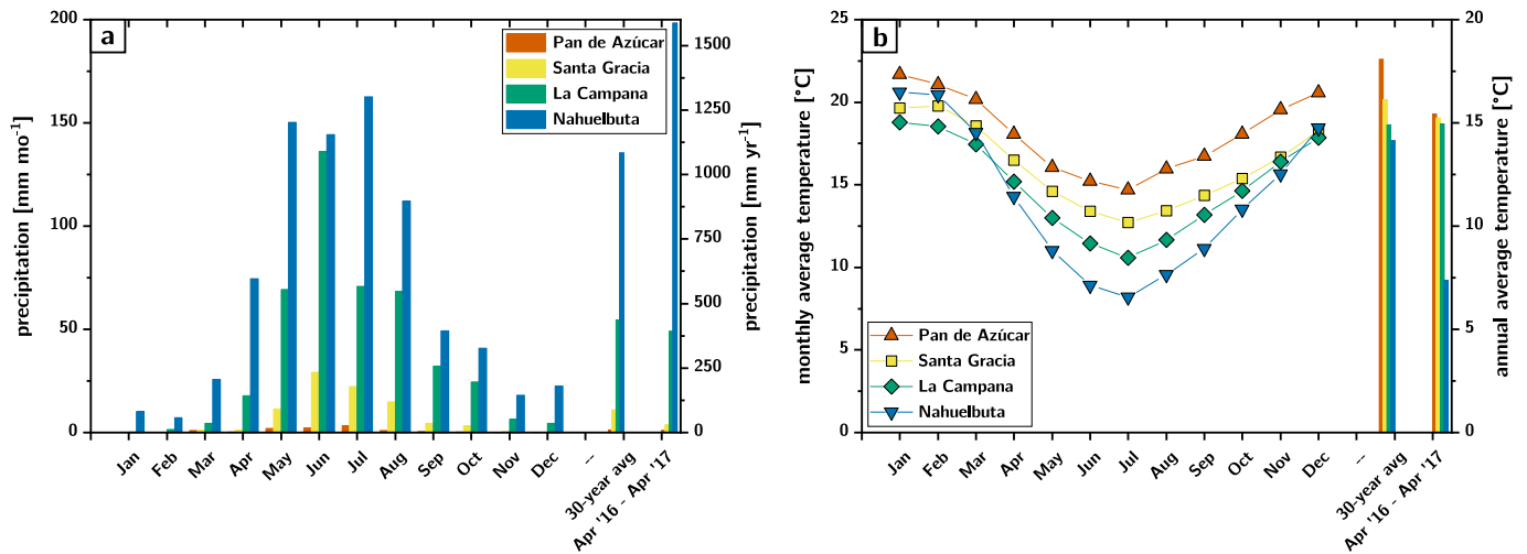
Fig. 2. Compilation of precipitation (A) and temperature (B) data from climate stations in vicinity of the respective EarthShape study sites (Ministerio de Obras Públicas, 2017). Bars on the very right-hand side of both panels show climate data from April 16 to April 17 at the EarthShape climate stations within the study sites (Ehlers et al., 2017).
