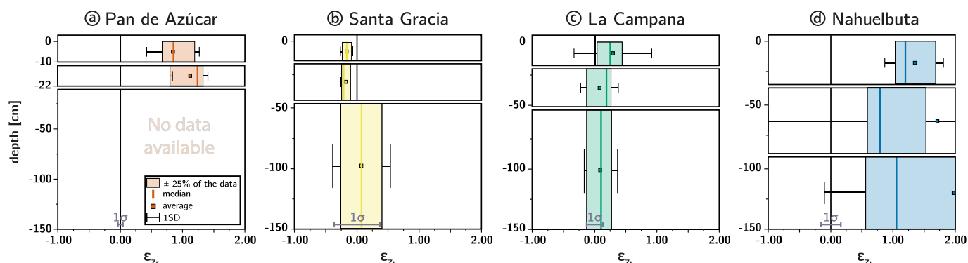
Fig. 13. Volumetric strain ( \epsilon ) for each study sites' averaged A horizon (top), B horizon (middle) and saporlite (bottom) samples. Positive values denote to expansion and negative values to collapse of the regolith profile. See legend in panel a for the explanation of the uncertainty bars. The accuracy of the absolute \epsilon values is limited by the variability in the respective sites' bedrock Zr concentration as indicated by the gray 1\sigma bar at the graphs' bottom. Note that the Y-axis scale is expanded by a factor of three for the A and B horizon in Pan de Azúcar. In this study site, no \epsilon is available for the saporlite, as bulk density has not been determined for these samples.
