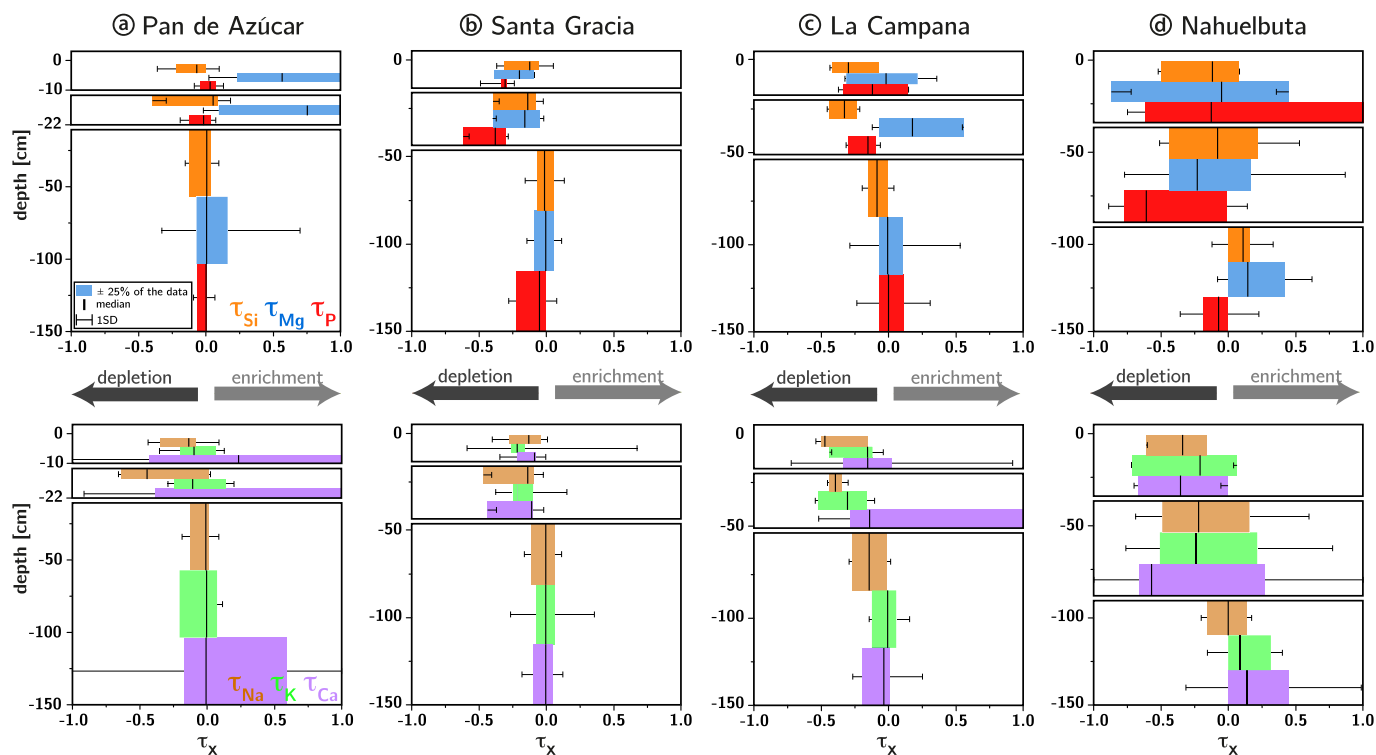
Fig. 12. Elemental mass transfer coefficient ( \tau , the fractional element loss that was calculated here relative to the sample at the base of the regolith profile) for each study sites' averaged A horizon (top box), B horizon (middle box), and saporlite (bottom box) samples. The upper graphs show \tau values for Si, Mg, and P, whereas the lower graphs show \tau values for Na, K, and Ca. Note that the shown \tau values are only stacked for visualization reasons and represent \tau values averaged over the study sites' specific horizons. Further, the Y-axis scale is expanded by a factor of three for the A and B horizon in Pan de Azúcar.
