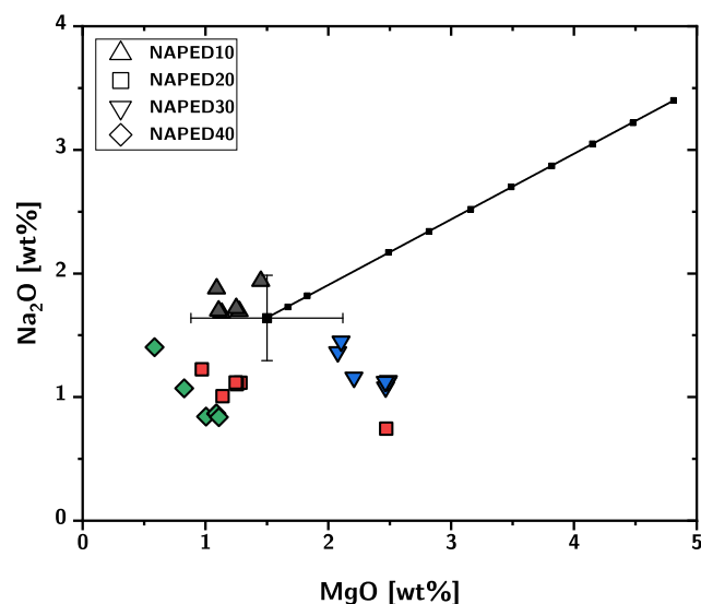
Fig. 17. Mixing model between average Na and Mg concentrations of Nahuelbuta saprolites ( \text{Na}_2\text{O} : 1.64 wt% and \text{MgO} : 1.50 wt%) and andesitic ash ( \text{Na}_2\text{O} : 3.40 wt% and \text{MgO} : 4.81 wt%), respectively. The black line represents the mixing line between 0% volcanic ash input to the left and 100% volcanic ash input to the right. Symbols represent samples from the A and B horizons at Nahuelbuta. The model indicates that the contribution of ash at the Nahuelbuta site is, if existing at all, insignificant.
