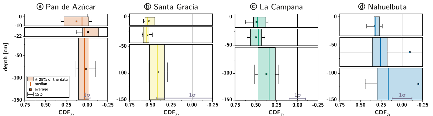
Fig. 11. Chemical Depletion Fraction (CDF) for each study sites' averaged A horizon (top), B horizon (middle) and sapolite (bottom) samples. See legend in panel a for the explanation of the uncertainty bars. The accuracy of the absolute CDF values is limited by the variability in the respective sites' bedrock Zr concentration as indicated by the gray 1 \sigma bar at the graphs' bottom. Note that the Y-axis scale is expanded by a factor of three for the A and B horizon in Pan de Azúcar.
