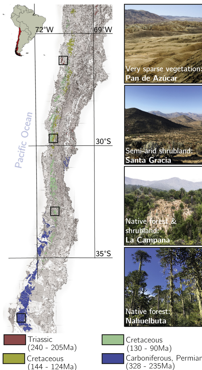
Fig. 1. Intrusion age and spatial extension of the granitoid rocks in the four primary EarthShape study sites (open squares) along the Chilean Coastal Cordillera from north to south: Pan de Azúcar, Santa Gracia, La Campana, and Nahuelbuta.
