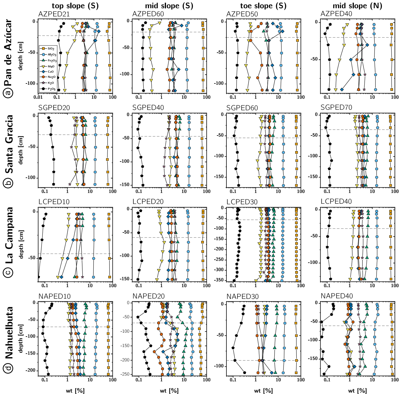
Fig. 8. Depth-dependent major element composition (corrected for LOI following Eq. (1)) of the four primary EarthShape study sites (regolith profile names indicated above). Differences between sites are attributed to large-scale bedrock variations and differences within the single catenae to small-scale lateral and vertical bedrock heterogeneities. Vertical variations within a profile (i.e. LCPED30, NAPED20, NAPED40) reflect a change in substrate. Dashed lines indicate the soil – saprolite boundary.
