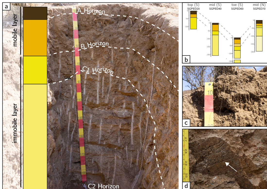
Fig. 4. Photographs of the S-facing mid slope pit (SGPED 40) in Reserva Natural Santa Gracia (SG) including horizon boundaries (white dashed line), a profile sketch, and a cross section through the S-facing catena and adjacent N-facing pit. The catena developed on a medium grain size granitic substrate. The regoliths' upper layer is characterized by bioturbation and a high root density (a). At the pits' base, two major joint sets are preserved. Here, roots penetrate the fractures and weather the adjacent rock face (b).
