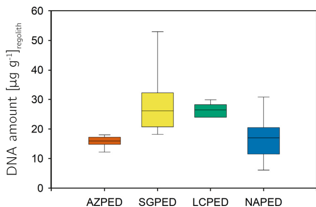
Fig. 15. Concentration of extracted DNA, averaged over the entire sampled saprolite depth. Box plots represent the sum of values of all topographic positions combined in Nahuelbuta (NAPED), La Campana (LCPED), Santa Gracia (SGPED) and Pan de Azúcar (AZPED). Median lines are indicated within the boxes of which the size corresponds to \pm 25\% of the data, whereas the whiskers show \pm 1 st dev of all data. DNA was extracted from saprolite samples in triplicates.
