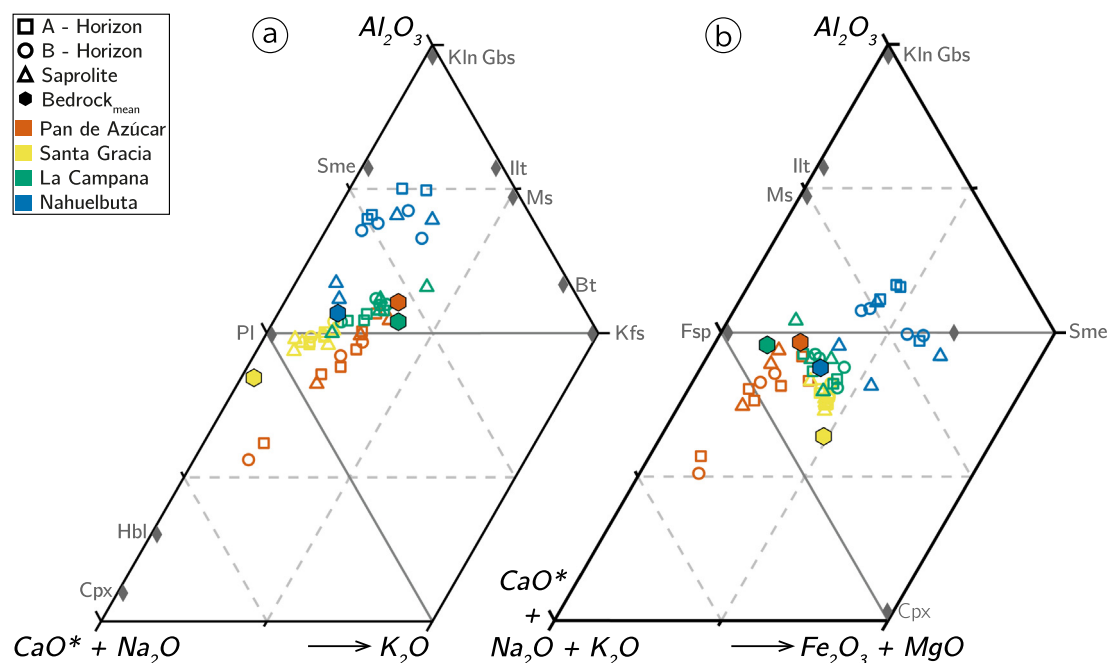
Fig. 9. Weathering trends for regolith profiles in Pan de Azúcar (red), Santa Gracia (yellow), La Campana (green), and Nahuelbuta (blue) in the ternary space of A-CN-K (a) and A-CN-K-FM (b) as introduced by Nesbitt and Young (1982) (molar proportions). Note that (a) corresponds to the CIA which is 100 at pure Al_2O_3 , and 50 at connecting line between Pl and Kfs. The gray diamonds represent idealized mineral compositions: Bt - biotite; Cpx - clinopyroxene; Fsp - feldspar; Gbs - gibbsite; Hbl - hornblende; Illt - illite; Kfs - K-feldspar; Kln - kaolinite; Ms - muscovite; Pl - plagioclase; Sme - smectite. (For interpretation of the references to color in this figure legend, the reader is referred to the web version of this article.)
