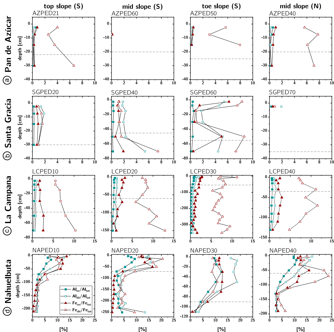
Fig. 14. Ratios of Al and Fe concentrations of the pedogenic oxide fraction (oxalate extracted, closed symbols; dithionite extract, open symbols) relative to total sample concentration. Regolith profile names are indicated above and dashed lines indicate the soil-saprolite boundary.
