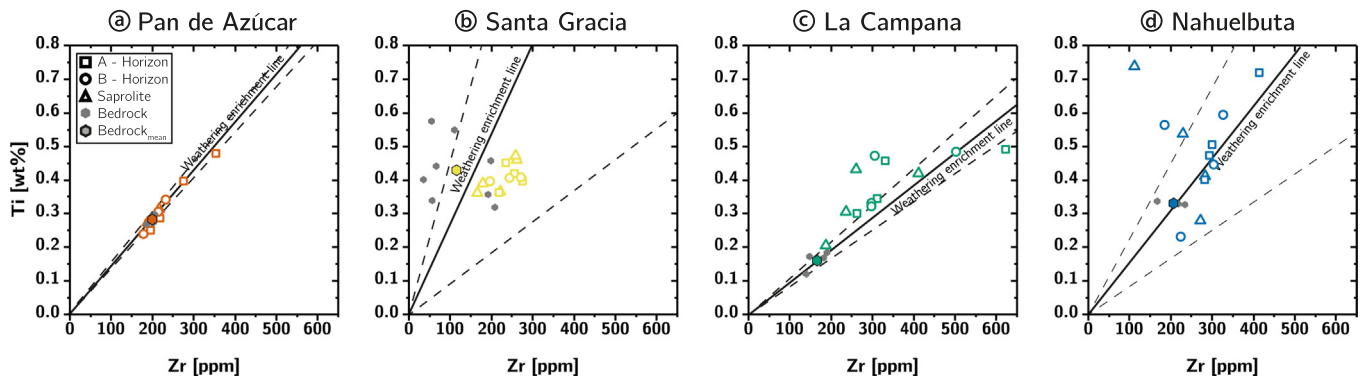
Fig. 10. Ti and Zr concentration measured in soil, sapolite, and bedrock at the four primary EarthShape study sites. Solid lines (with error envelope, dashed) indicate the weathering enrichment line for bedrock composition, constructed from initial element ratios from bedrock samples and their uncertainty, as quantified by the Ti and Zr concentration of multiple bedrock samples.
