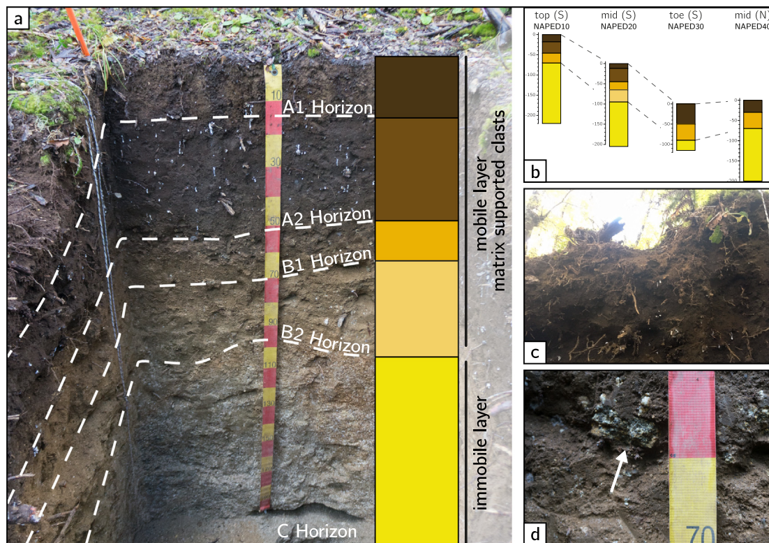
Fig. 6. Photographs of the S-facing mid slope pit (NAPED 20) in Parque Nacional Nahuelbuta (NA) including horizon boundaries (white dashed line), a profile sketch, and a cross section through the S-facing catena and adjacent N-facing pit. Very high organic matter content, characterize the upper horizons of the four pits (a). Fragments are absent in the regoliths' A-Horizon; they occur in the B-Horizon in the form of weathered granodiorite (b). Rare fragments of mafic composition are also found.
