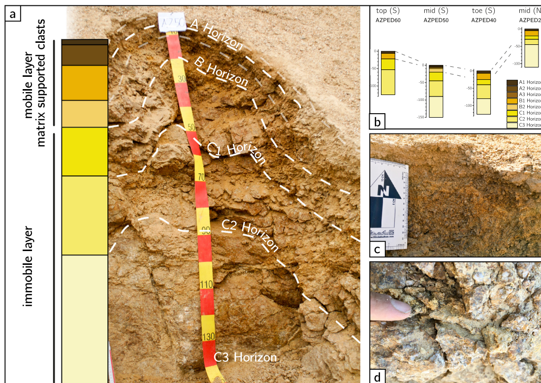
Fig. 3. Photographs of the S-facing mid slope regolith profile (AZPED 50) in Parque Nacional Pan de Azúcar (AZ) including horizon boundaries (white dashed line), a schematic depth profile (a), a cross section through the S-facing catena and adjacent N-facing regolith profile (b). The regolith in AZ developed on a coarse-grained, feldspar-rich granite. Its cover lacks fine-grained particles which are removed by wind (c). Fractures are either filled with clay-sized particles of unknown composition or gypsum and carbonate (d).
