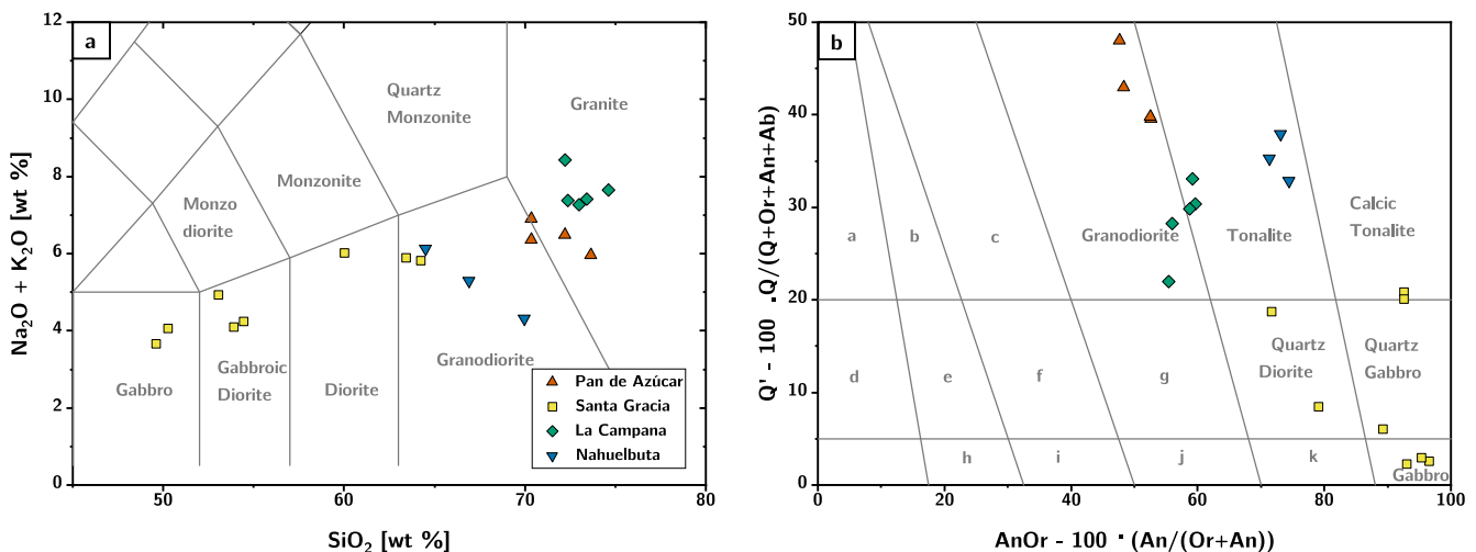
Fig. 7. Classification diagrams for siliceous igneous and volcanic rocks. (a) Total alkali versus silica diagram introduced by Le Bas et al. (1986). (b) Q-AnOr diagram of Streckeisen and LeMaitre (1979), where the mineral modes were determined from XRF analyses by the CIPW norm calculation. Field association as follows: a - Alkali-feldspar granite; b - Syenogranite; c - Monzogranite; d - Alkali-feldspar Quartz Syenite; e - Quartz Syenite; f - Quartz Monzonite; g - Quartz Monzodiorite; h - Syenite; i - Monzonite; j - Monzogabbro; k - Diorite.
