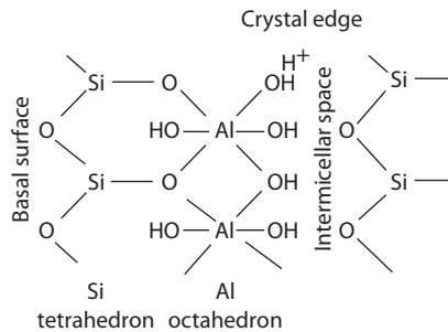
FIGURE 9.1 Protonation of structural aluminol groups.
