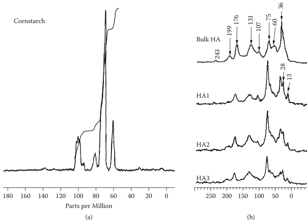
FIGURE 5.28 Evidence of the presence of polysaccharides in the humic acid fractions of Conte et al. (2006). (a) Solid-state cross-polarization magic-angle-spinning carbon-13 nuclear magnetic resonance (CP-MAS ^{13}\text{C} -NMR) spectrum of polysaccharide (cornstarch), analysis. (D. Himmelsbach, U.S. Department of Agriculture Agricultural Research Service, Athens, GA.) (b) Solid-state CP-MAS ^{13}\text{C} -NMR of bulk HA (humic acid) and its eluted high-performance size-exclusion chromatography (HPSEC) fractions HA1, 2, and 3 from Conte and coworkers. Only three of the 11 fractions are shown here. The main NMR signal at 60 to 80 ppm was shown to increase in intensity from HA3 to HA1 and was the dominant signal of the spectra. (From Conte, P., R. Spaccini, and A. Piccolo, Anal. Bioanal. Chem. 386(2), 382–390, 2006. With permission.)
