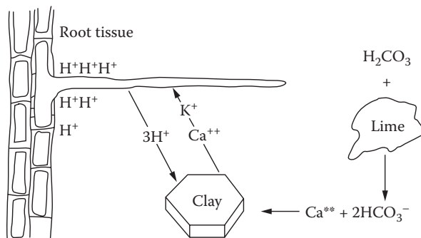
FIGURE 8.1 Cation exchange involving a mixture of mono- and polyvalent ions by a soil colloid with a certain amount of charges: Ca^{2+} and K^+ on the clay surface are exchanged for 3 H^+ by plant roots.
