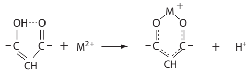
FIGURE 12.3 Example of formation of metal ( M^+ ) chelate ring structure.
