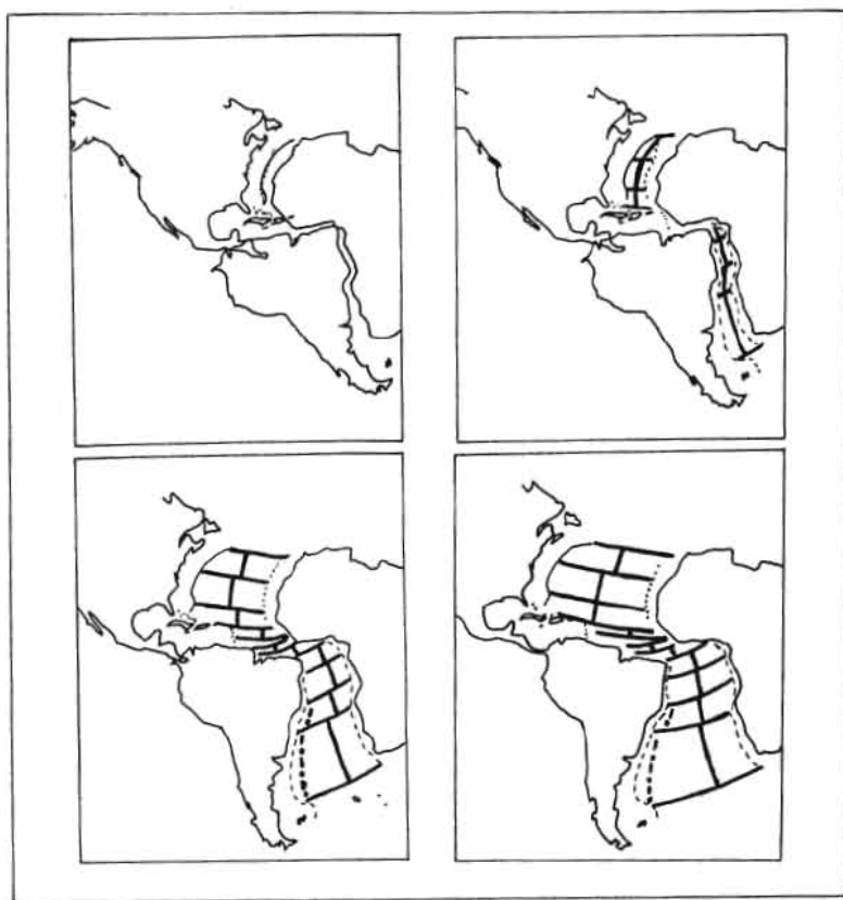
Fig. 10. The Mesozoic episode of spreading in the Atlantic. These reconstructions were obtained by assuming that North and South America parted simultaneously from Africa 120 m.y. ago (upper left) and reached the position corresponding to anomaly 31 (Figure 9) about 90 m.y. ago (lower right) after a single movement of rotation for each. The asymmetry of the ridge crest in the South Atlantic at the time of anomaly 31 is explained by a shift in the ridge crest positions in the Early Cretaceous. The fit is made to the 'quiet' magnetic zone boundaries in the North Atlantic and to the 500-fathom line in the South Atlantic [Bullard et al. , 1965]. See Table 7. The active ridge crests and fracture zones are represented by a thick continuous line, the abandoned ridge crest by a thick dash-dot line.
