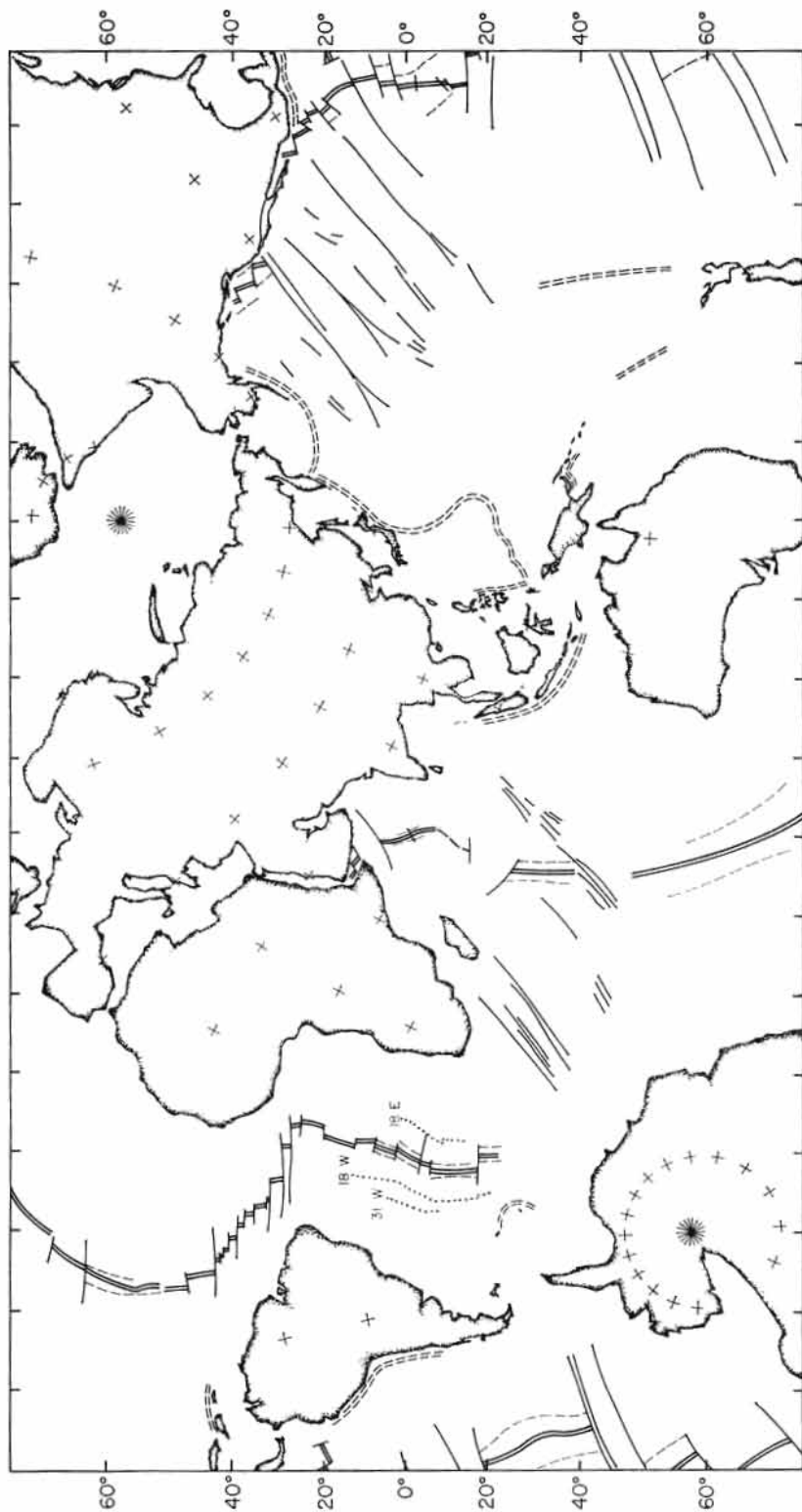
Fig. 3. The pole of projection has been shifted to the Atlantic Ocean center of rotation (58°N, 37°W).
