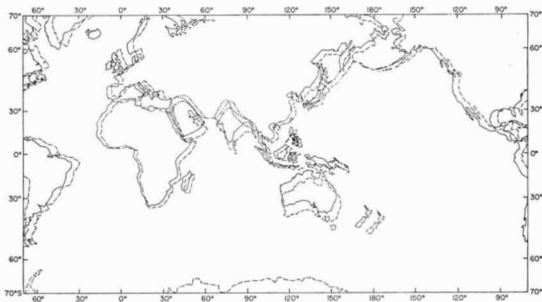
Fig. 7. The positions of the continents at the time of anomaly 5 ( \approx 10 m.y. ago) with respect to Antarctica are shown by dashed lines, the present positions of the continents by full lines. The present northern boundaries of Arabia and India are shown by dotted lines, and the dash-dot lines define the gap which results from the rotations back to 10 m.y. ago.
