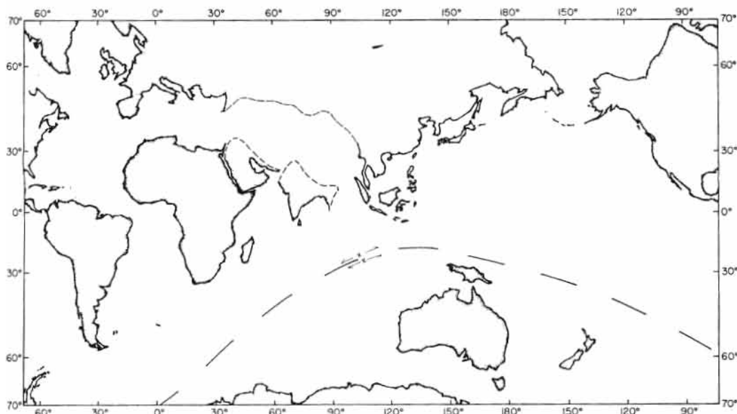
Fig. 8. The positions of the continents at the time of anomaly 31 (Paleocene). The dashed line indicates that the relative positions of the two groups of continents on each side of it were not known: Antarctica and Africa are assumed to have been in their present positions. See text and Table 7 for details.
