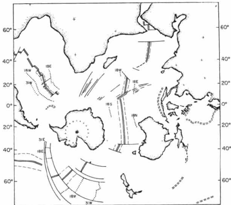
Fig. 4. The pole of projection has been shifted to the Indian Ocean center of rotation ( 26^{\circ}\text{N} , 21^{\circ}\text{E} ).
