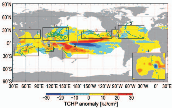
FIG. 4.26. Global anomalies of TCHP corresponding to 2009 computed as described in the text. The boxes indicate the seven regions where TCs occur: from left to right, Southwest Indian, North Indian, West Pacific, Southeast Indian, South Pacific, East Pacific, and North Atlantic (shown as Gulf of Mexico and tropical Atlantic separately). The green lines indicate the trajectories of all tropical cyclones reaching at least Cat-1 (1-minute average maximum wind \geq 119 km hr -1 ) and above during November 2008–December 2009 in the Southern Hemisphere and 2009 in the Northern Hemisphere. The numbers above each box correspond to the number of Cat-1 and above cyclones that travel within each box. The Gulf of Mexico conditions during June–November 2009 are shown in detail in the insert shown in the lower right corner.
