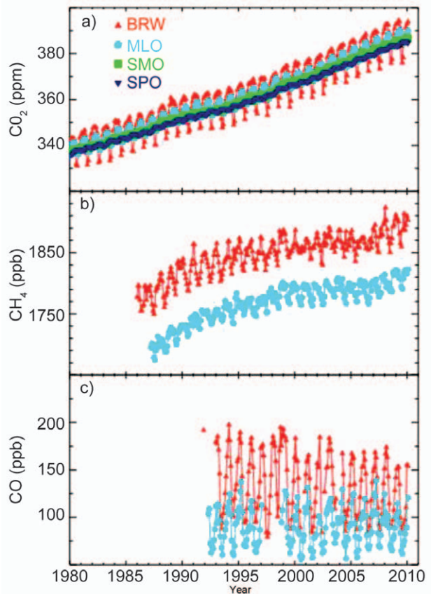
FIG. 2.35. Monthly mean mole fractions determined from NOAA/ESRL Observatories at Barrow, Alaska (BRW); Mauna Loa, Hawaii (MLO); American Samoa (SMO); and South Pole (SPO) for (a) CO 2 , (b) CH 4 , and (c) CO. 2009 results are preliminary. Monthly means are courtesy of Kirk Thoning (CO 2 ), Ed Dlugokencky (CH 4 ), and Paul Novelli (CO), all from NOAA/ESRL. Additional plots can be found at http://www.esrl.noaa.gov/gmd/ccgg/iadv/ and http://www.esrl.noaa.gov/gmd/Photo_Gallery/GMD_Figures/ccgg_figures/ .
