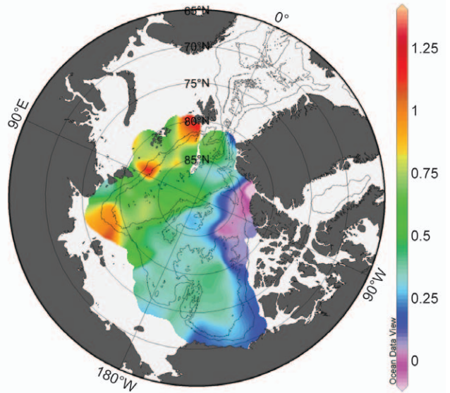
FIG. 5.8. 2007–09 Atlantic water layer temperature maximum anomalies relative to climatology of Timokhov and Tanis (1997, 1998).
