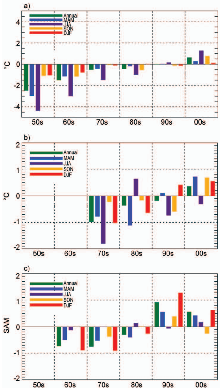
FIG. 6.1. Decadal averages of the seasonal and annual mean anomalies for (a) temperature at Faraday/Vernadsky, (b) temperature at Marambio, and (c) SAM index ( http://www.antarctica.ac.uk/met/gjma/sam.html ). See Fig. 6.4a for locations of stations used in 6.1a–b.
