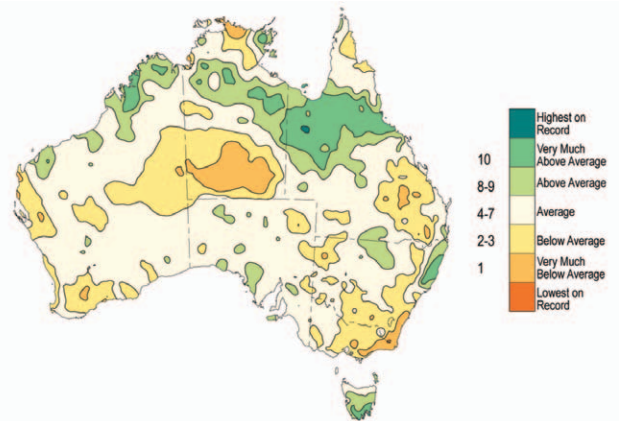
FIG 7.51. Australian annual rainfall deciles (since 1900) for 2009.
