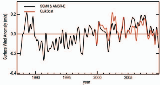
FIG. 2.31. Surface wind speed anomalies over the global ice-free oceans as measured by Remote Sensing Systems from the SSM/I and the Advanced Microwave Scanning Radiometer EOS (AMSR-E) instruments. The time series has been smoothed to remove variability on time scales shorter than 4 months. The reference period for the combined AMSR-E and SSM/I measurements is 1988–2007. For the QuikSCAT measurements the reference period is 2000–2007, with the mean adjusted to match the SSM/I anomalies for 2000–07.
