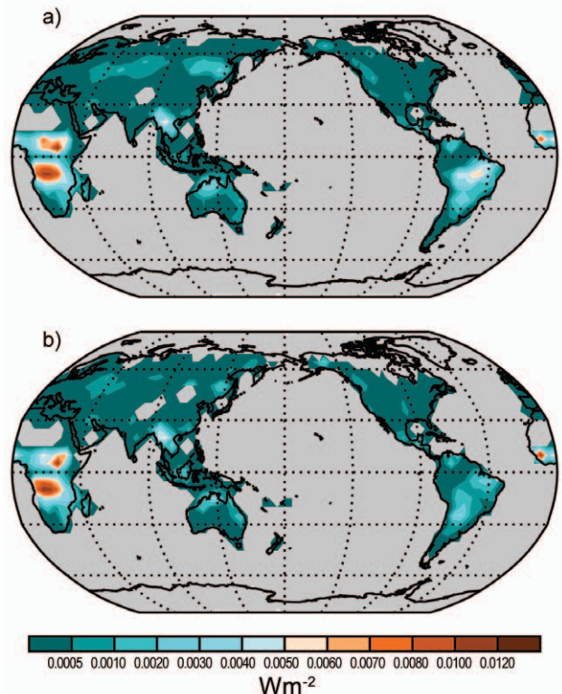
FIG. 2.49. Global fire distribution of 2003–08 (climatological period) (a) and 2009 (b), all in terms average fire radiative power density ( W m^{-2} ) observed by MODIS.
