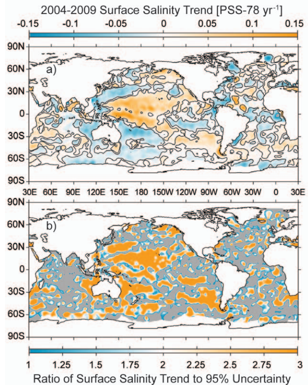
FIG. 3.14. (a) Map of local linear trends estimated from annual surface salinity anomalies for the years 2004–09 estimated from Argo data (colors in PSS-78 yr -1 ). (b) The ratio of these trends to estimates of the 95% confidence interval, with grey regions showing areas without statistically significant trends and colors from blue to orange indicating increasing statistical significance of the trends.
