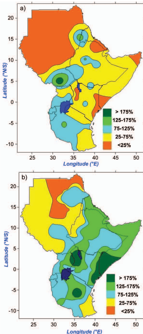
FIG. 7.21. (a) December 2008 to February 2009 rainfall anomalies and (b) October to December 2009 rainfall anomalies (expressed as percentage of 1961–90) for the Great Horn of Africa. (Source: ICPC, 2009.)
