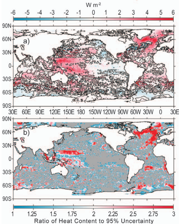
FIG. 3.6. (a) Linear trend from 1993 to 2009 of the combined satellite altimeter and in situ ocean temperature data estimate of upper (0–750 m) ocean heat content anomaly OHCA ( \text{W m}^{-2} ) analyzed following Willis et al. (2004). (b) Ratio of the linear trend to its 95% uncertainty estimate, with colored areas showing regions with statistically significant trends, and grey areas those without.
