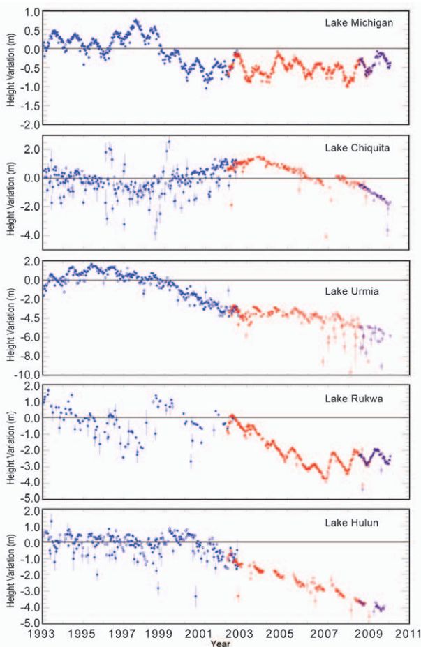
FIG. 2.25. Lake level products from the NASA/USDA/FAS. Topex/Poseidon (blue), Jason-1 (red), and Jason-2 (purple) radar altimeters. The lakes reside in the United States (Michigan), Argentina (Chiquita), Iran (Urmia), Tanzania (Rukwa), and China (Hulun).
