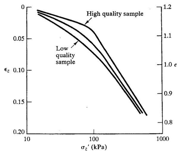
Effect of sample disturbance on consolidation test results.
