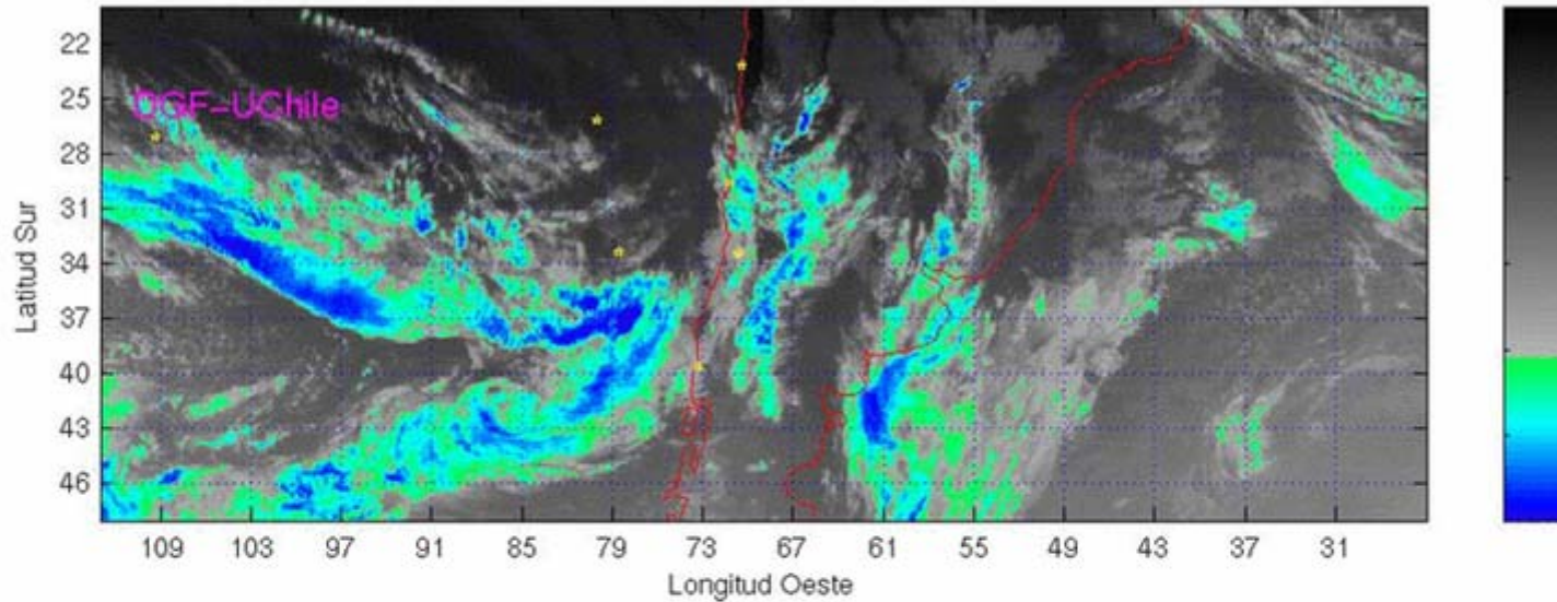
GOES-8 Canal IR2
