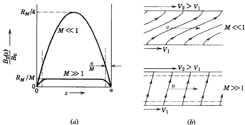
Fig. 10.3 (a) Axial component of magnetic induction between the boundary surfaces for large and small Hartmann numbers. (b) Transport of lines of magnetic induction in direction of flow.
