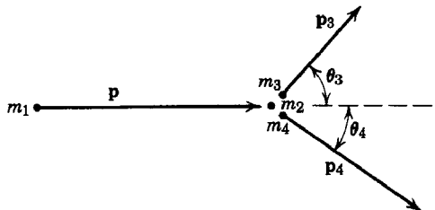
Fig. 12.3 Momentum vectors in laboratory for a two-body process.
