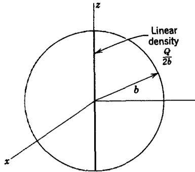
Fig. 3.10 Uniform line charge of length 2b and total charge Q inside a grounded, conducting sphere of radius b .
