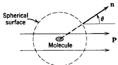
Fig. 4.11 Calculation of the internal field—contribution from distant molecules.
