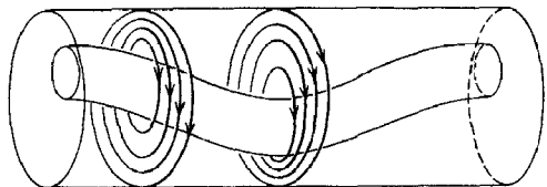
Fig. 10.11 Stabilization of long-wavelength kinks with outer conductor.
