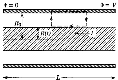
Fig. 10.6 Plasma column inside a hollow, cylindrical conductor.
