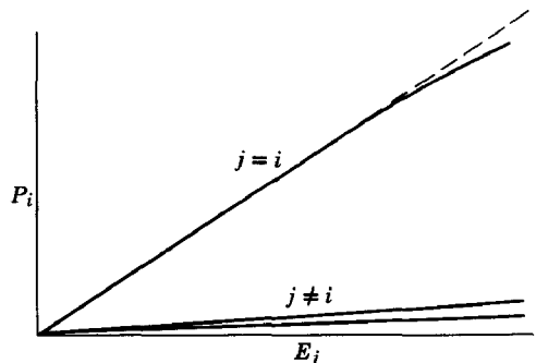
Fig. 4.3 Components of polarization as a function of applied electric field.
