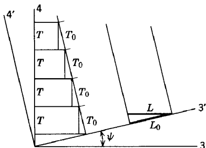
Fig. 11.12 Time dilation and Fitzgerald-Lorentz contraction in terms of a rotation of space-time axes.
