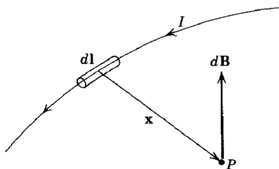
Fig. 5.1 Elemental magnetic induction d\mathbf{B} due to current element I dl .
