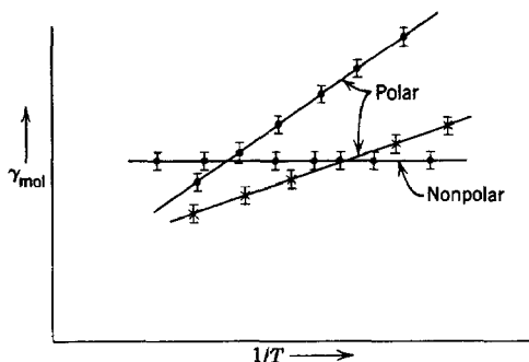
Fig. 4.13. Variation of molecular polarizability \gamma_{mol} with temperature for polar and non-polar substances. \gamma_{mol} is plotted versus T^{-1} .
