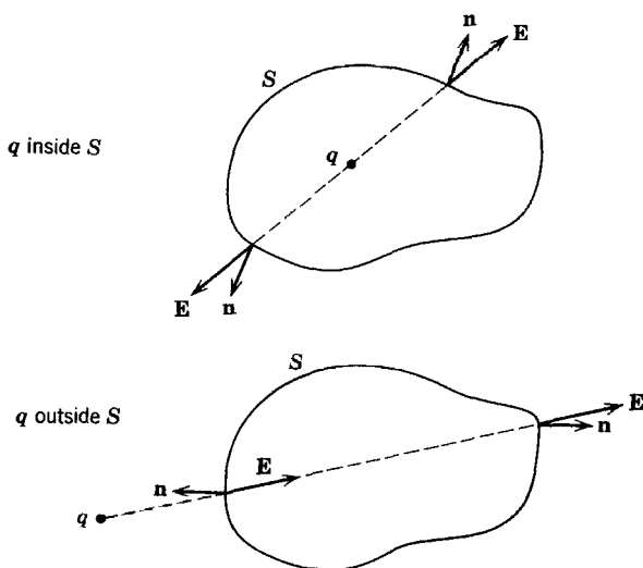
Fig. 1.2 Gauss's law. The normal component of electric field is integrated over the closed surface S . If the charge is inside (outside) S , the total solid angle subtended at the charge by the inner side of the surface is 4\pi (zero).
