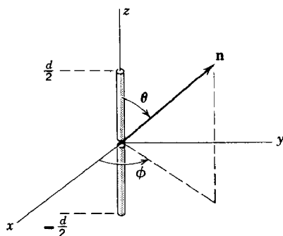
Fig. 9.1 Short, center-fed, linear antenna.
