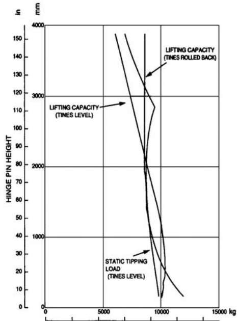
STATIC TIPPING LOAD (STRAIGHT) AND LIFTING CAPACITY
