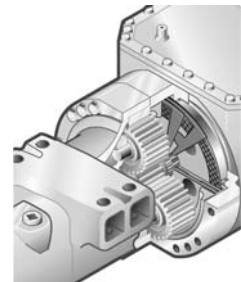
Wet type disc parking brake
