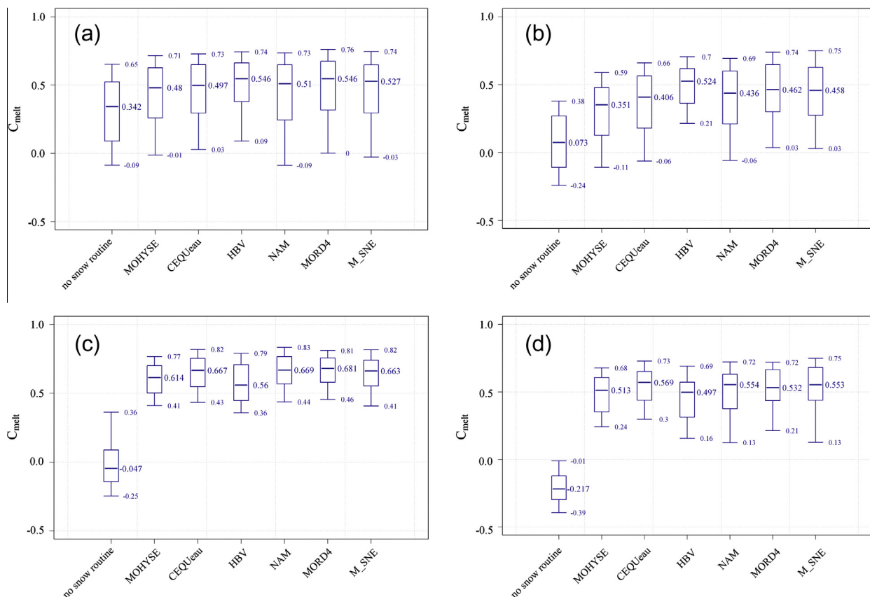
Fig. 4. Box plots (showing 0.10, 0.25, 0.50, 0.75 and 0.90 percentiles) of the distributions of C_{melt} criteria obtained in validation by the HBV9 model without any SAR and with one of the six SARs on (a) the 159 moderately snow-affected French catchments, (b) the 90 Swiss and French Alpine catchments, (c) the 94 Swedish catchments and (d) the 36 Canadian catchments.
