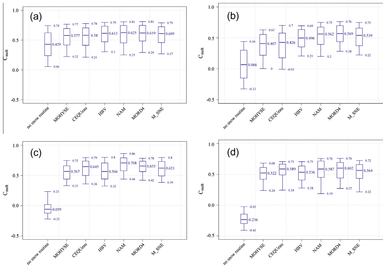
Fig. 3. Box plots (showing 0.10, 0.25, 0.50, 0.75 and 0.90 percentiles) of the distributions of C_{melt} criteria obtained in validation by the GR4J model without any SAR and with one of the six SARs on (a) the 159 moderately snow-affected French catchments, (b) the 90 Swiss and French Alpine catchments, (c) the 94 Swedish catchments and (d) the 36 Canadian catchments.
